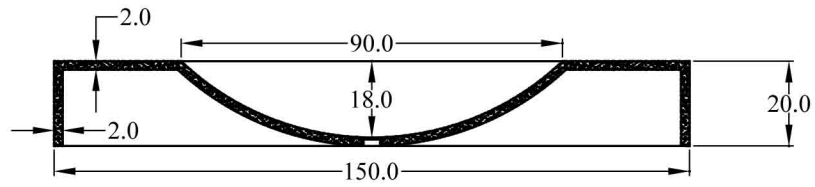
PLAN - SECTION
